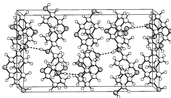
Figure 3. View of the elemental unit of (1 S ,2 S ,5 S ,6 S )-(–)-9-oxabicyclo[3.3.1]nonane-2,6-diol (–)- 3 along the y -axis
