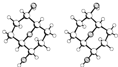
Figure 2. Stereoview of (1 S ,2 S ,5 S ,6 S )-(–)-9-oxabicyclo[3.3.1]nonane-2,6-diol [(–)- 3 ]
