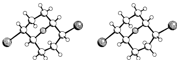
Figure 5. Stereoview of endo,endo -(±)-2,6-diiodo-9-oxabicyclo[3.3.1]nonane [(±)- 8 ]
