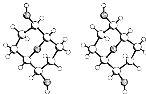
Figure 8. Stereoview of (1 S ,2 R ,5 S ,6 R )-(+)-9-oxabicyclo[3.3.1]nonane-2,6-diol [(+)- 12 ]
