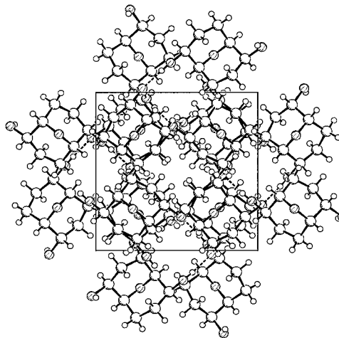
Figure 4. View of the elemental unit of (1 S ,2 S ,5 S ,6 S )-(–)-9-oxabicyclo[3.3.1]nonane-2,6-diol (–)- 3 along the z -axis
