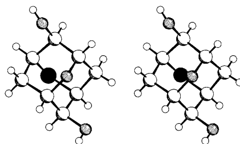
Figure 7. Stereoview of (1 S ,2 S ,4 S ,5 S ,7 S ,8 S )-(+)-2-oxa-6-thiaadamantane-4,8-diol (+)- 11
