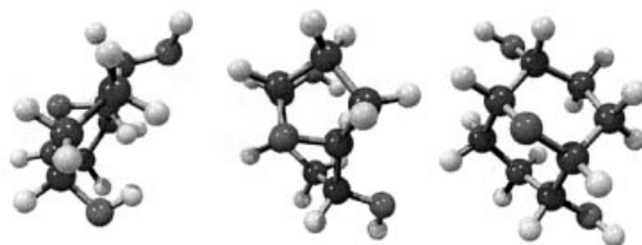
Figure 10. Comparison of the projections of the (5 S )- and the (2 R )-centers of meso - 2 with (2 R ,6 R )- 3
