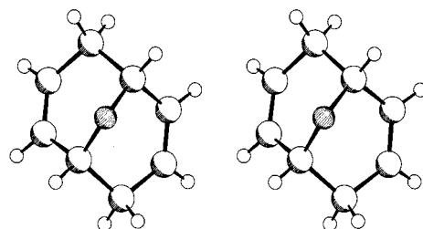
Figure 6. Stereoview of (±)-9-oxabicyclo[3.3.1]nona-2,6-diene [(±)- 9 ]
